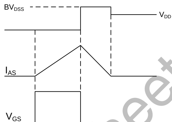
Fig.8 EAS Waveform
