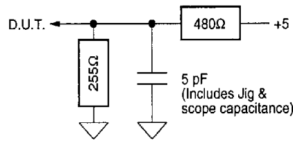
Figure 1b. Output Disable Timing Load
