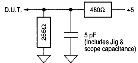
Figure 1b. Output Disable Timing Load
