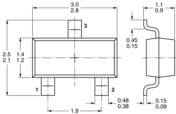
Fig 11. Package outline SOT23 (TO-236AB)
