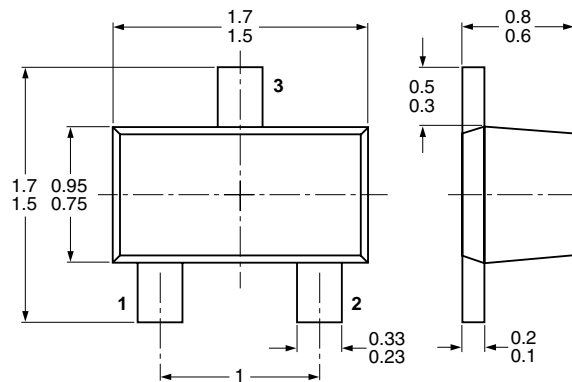
Fig 12. Package outline SOT323 (SC-70)
