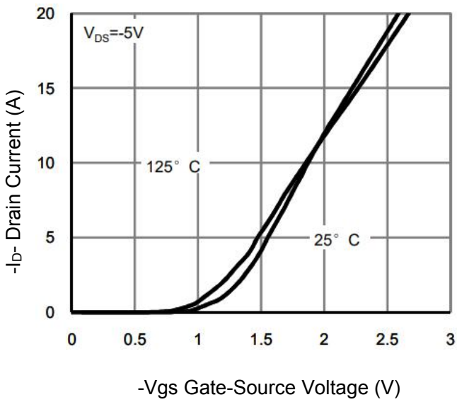
Figure 7 Transfer Characteristics
