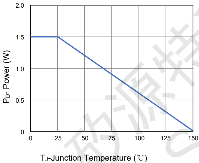
Figure 3 Power De-rating
