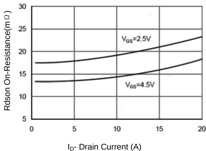
Figure 6 Drain-Source On-Resistance
