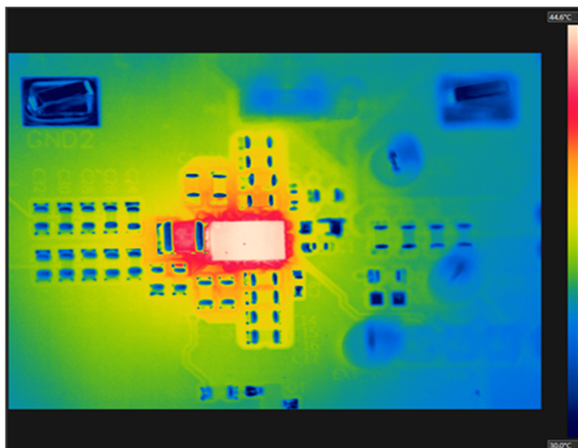
Figure 30. Thermal plot divide-by-2 I_{OUT} = 4A , ( V_{IN} = 7.7V and V_{OUT} = 3.72V ) P_{DISS} = 0.56W , top case temperature = 44.6^{\circ}C at T_A = 25^{\circ}C
