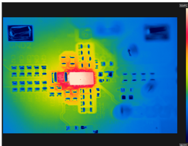
Figure 31. Thermal plot divide-by-3 I_{OUT} = 4A , ( V_{IN} = 11.55V and V_{OUT} = 3.62V ) P_{DISS} = 0.99W , top case temperature = 53.4^{\circ}C at T_A = 25^{\circ}C
