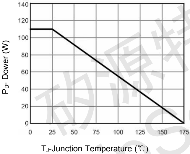
Figure 3 Power De-rating
