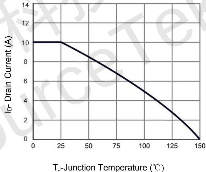
Figure 4 Drain Current
