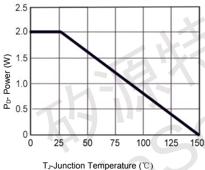
Figure 3 Power De-rating
