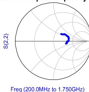
Figure 9. S22 vs. Output Frequency (VDD = 3 V)
