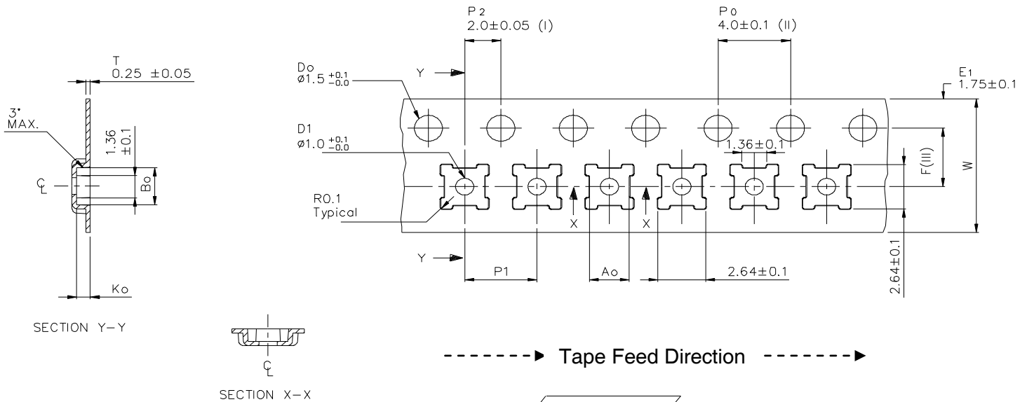
Figure 33. Tape and Reel Specifications 12-lead 2 x 2 x 0.55 mm QFN
