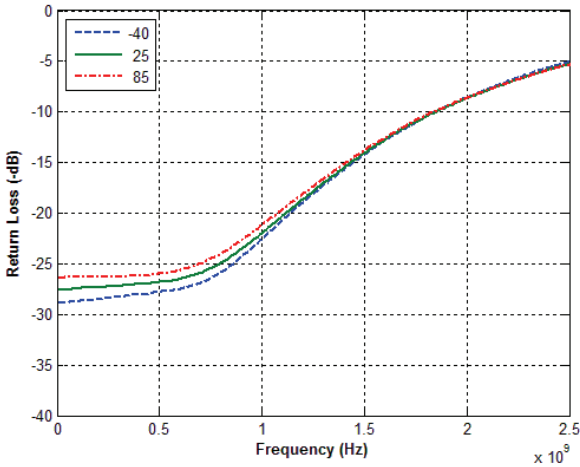
Figure 17. Return Loss vs. Temp (RX, Un-Attenuated)
