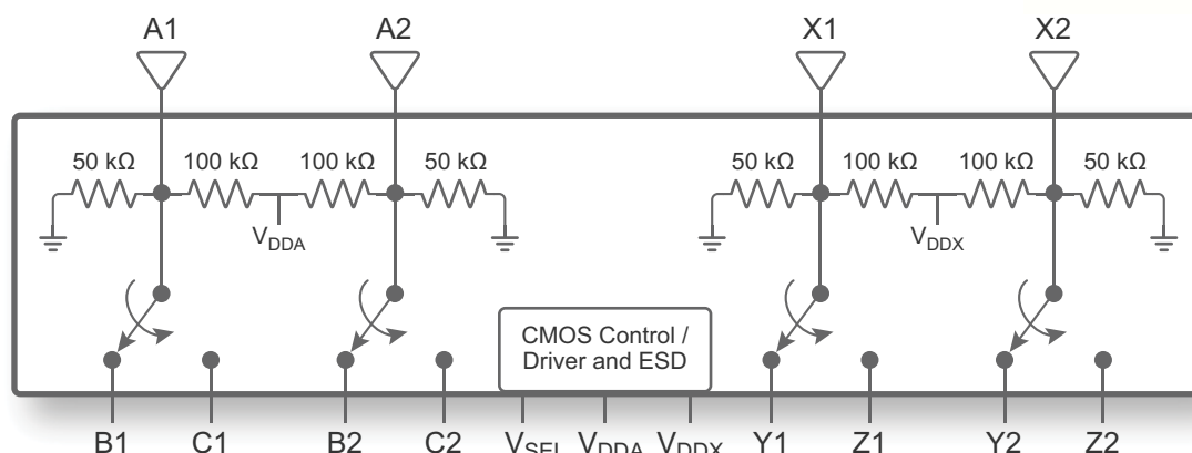
Figure 1. Functional Diagram
