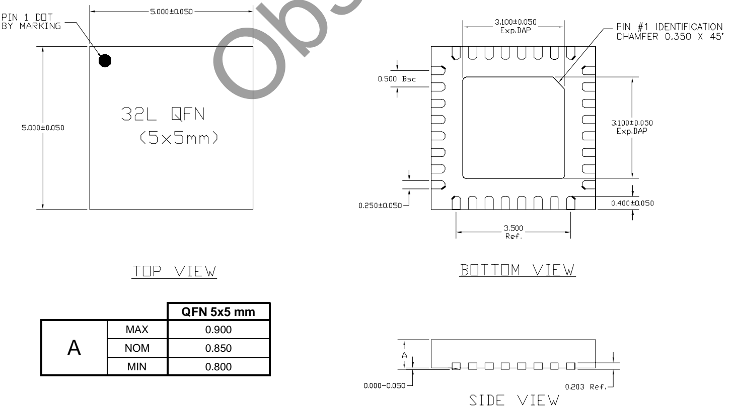
Figure 24. Package Drawing
