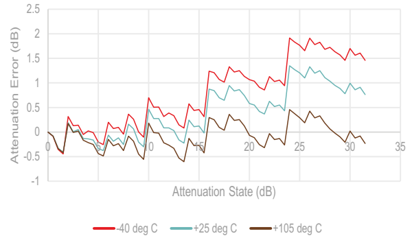
Figure 25 ■ Attenuation Error @ 43.5 GHz vs. Temperature
