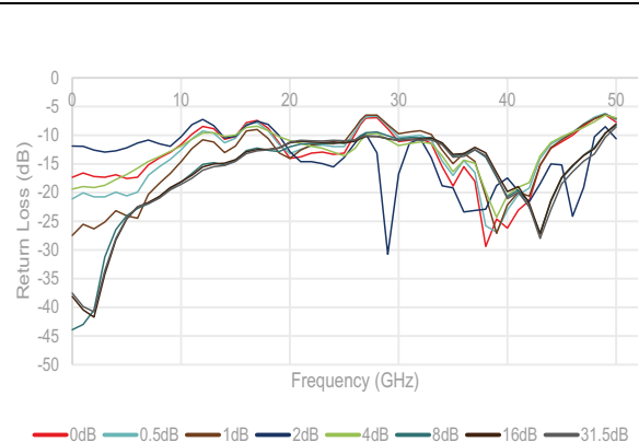
Figure 13 ■ Input Return Loss (Major Attenuation States)
