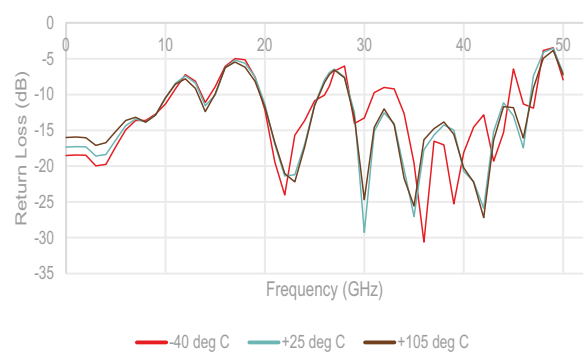
Figure 13 ■ Input Return Loss (Major Attenuation States)
