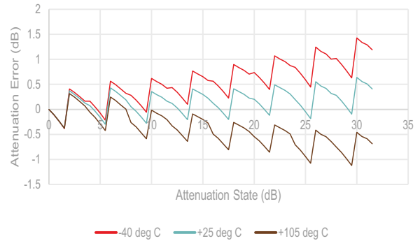
Figure 23 ■ Attenuation Error @ 26.5 GHz vs. Temperature
