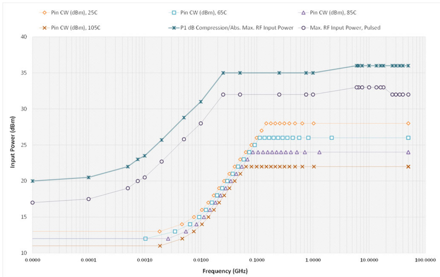
Figure 7 ■ Power De-rating Curve, 9 kHz–45 GHz, 50 Ohm
