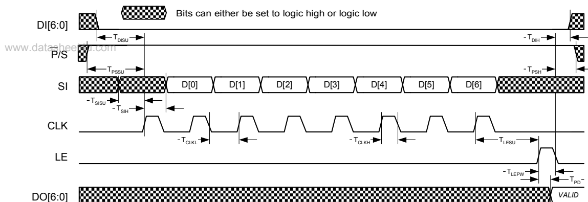
Figure 15. Serial Timing Diagram
