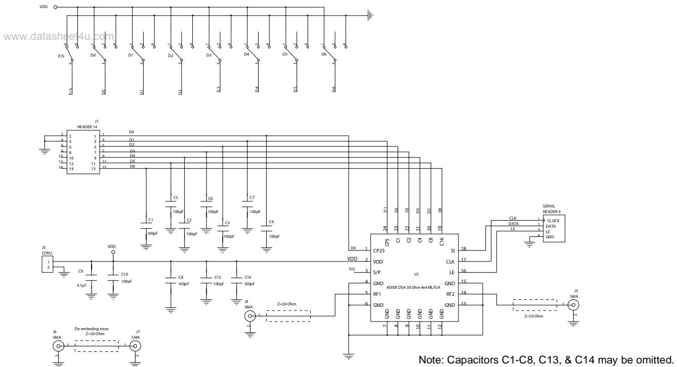
Figure 18. Evaluation Board Schematic Peregrine Specification 102-0379
