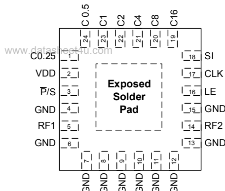
Figure 13. Pin Configuration (Top View)
