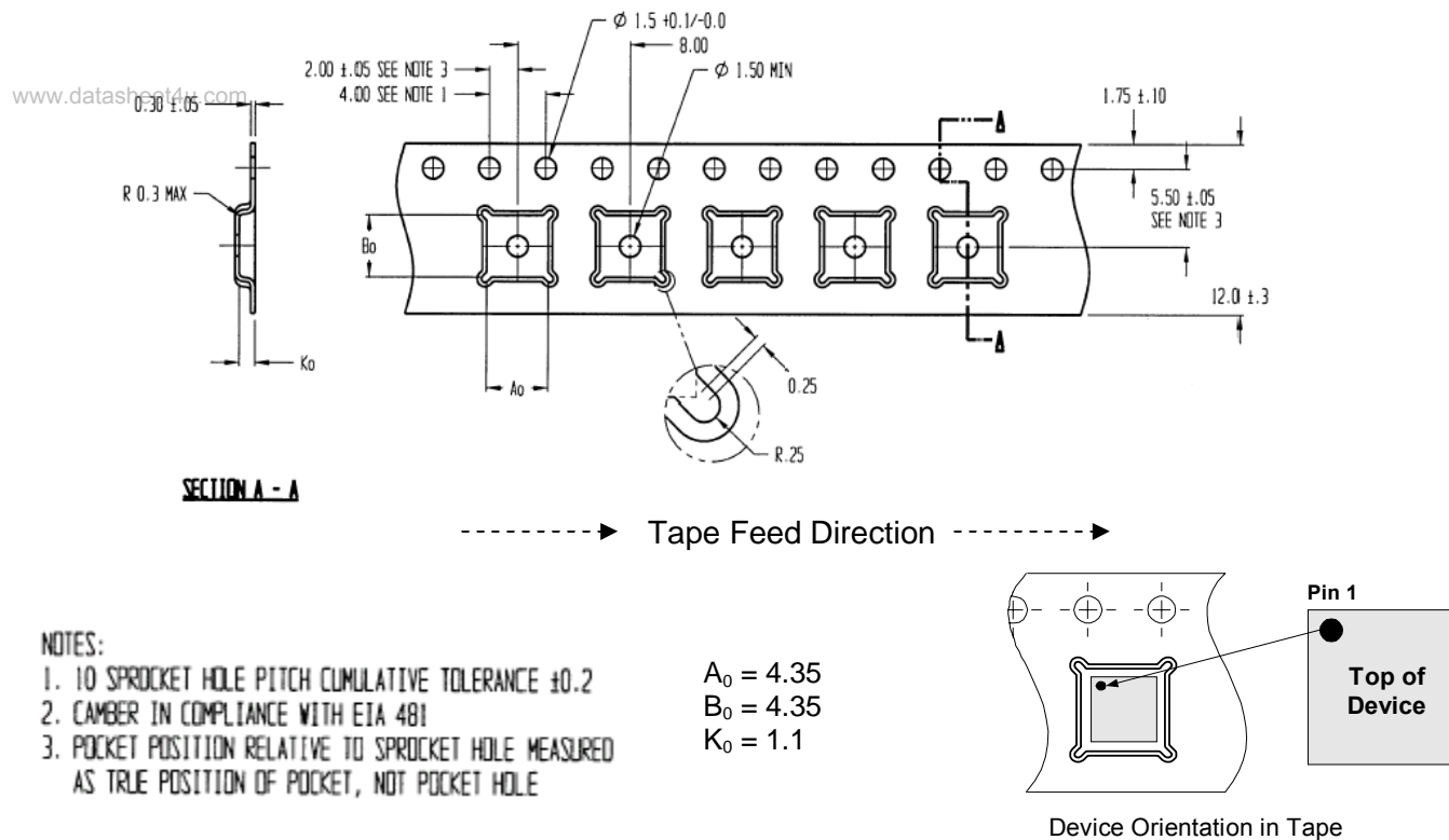
Figure 20. Tape and Reel Drawing
