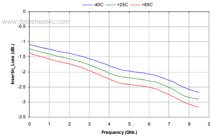
Figure 7. Insertion Loss vs. Temperature
