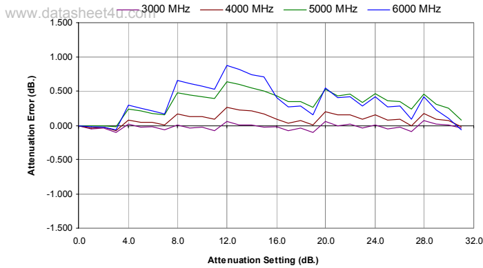
Figure 15. 1 dB Attenuation Error vs. Frequency
