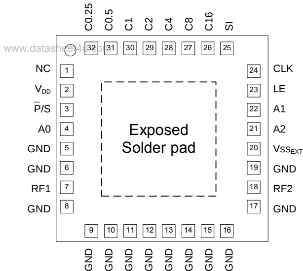
Figure 27. Pin Configuration (Top View)
