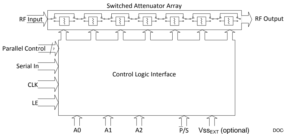
Figure 2. Functional Diagram
