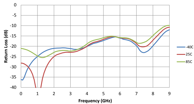
Figure 23. Output Return Loss vs. Temperature for 16 dB Attenuation Setting
