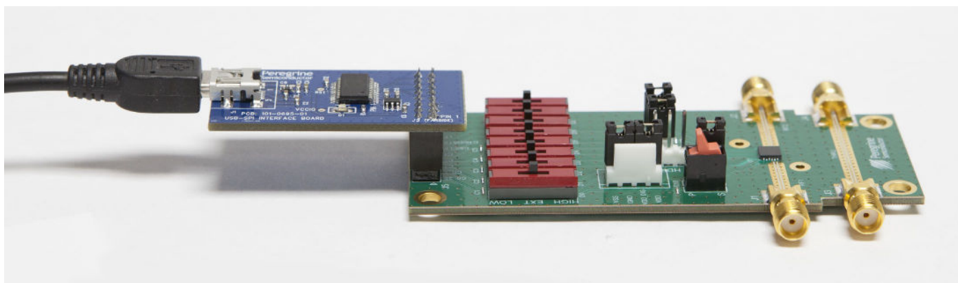
Figure 33 ■ Evaluation Kit for PE43711
