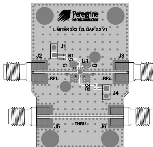
Figure 16. Evaluation Board Layout
