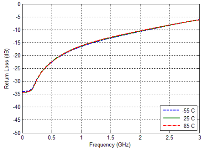
Figure 6. Input Return Loss vs. Temperature
