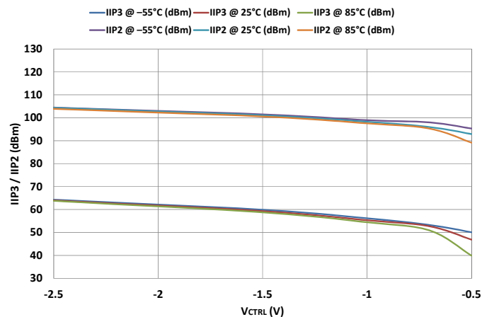
Figure 12. IIP3 / IIP2 vs. V_{CTRL} Over Temperature
