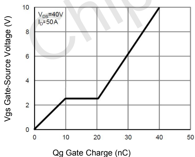
Figure 11 Gate Charge
