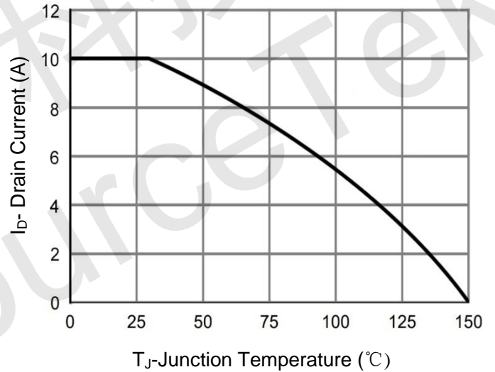
Figure 4 Drain Current
