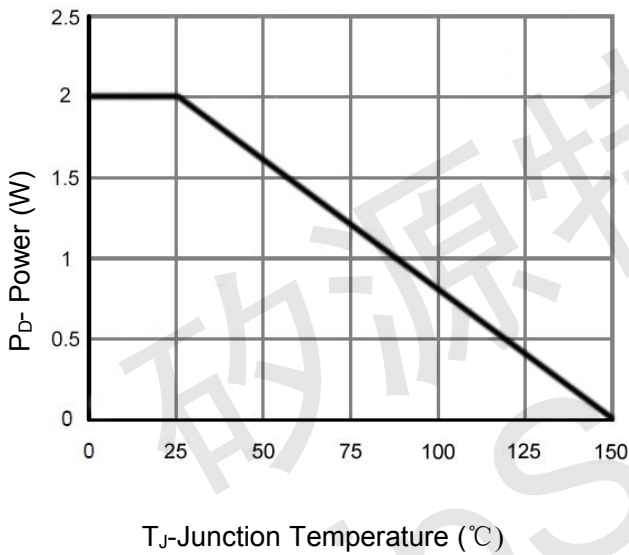
Figure 3 Power De-rating
