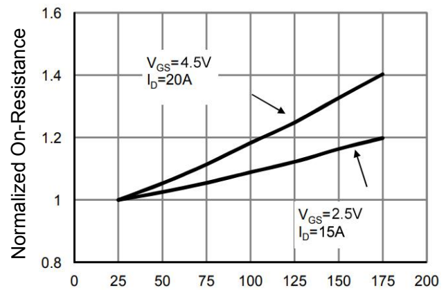
Tc-Case Temperature (°C) Figure 8 Rdson vs Junction Temperature
