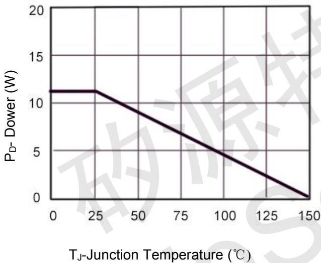
Figure 3 Power De-rating
