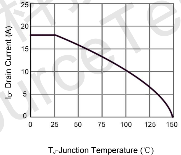
Figure 4 Drain Current
