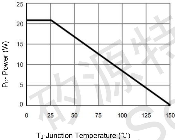
Figure 3 Power De-rating
