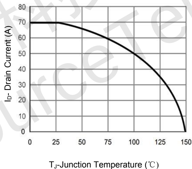
Figure 4 Drain Current
