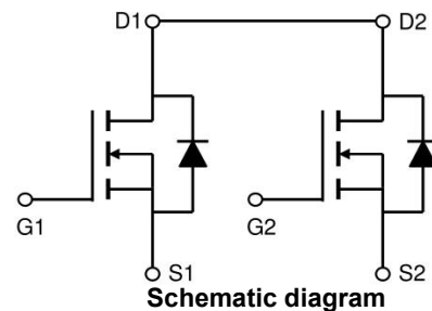
Schematic diagram
