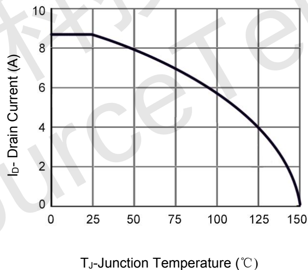
Figure 4 Drain Current
