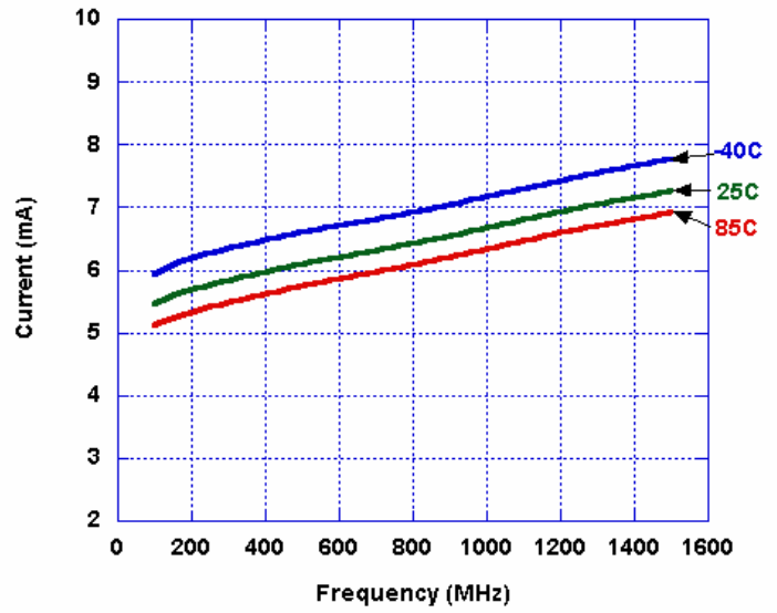
Figure 5. Device Current
