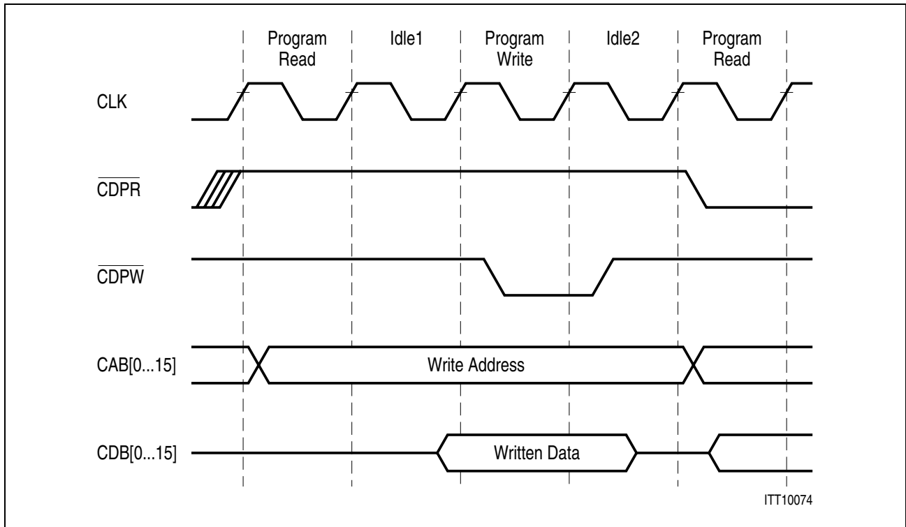
Figure 2-36 External Program Write Access Due to MOVD
