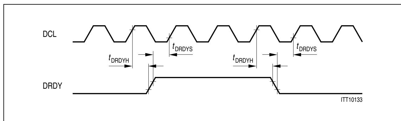
Figure 7-19 DRDY Timing
