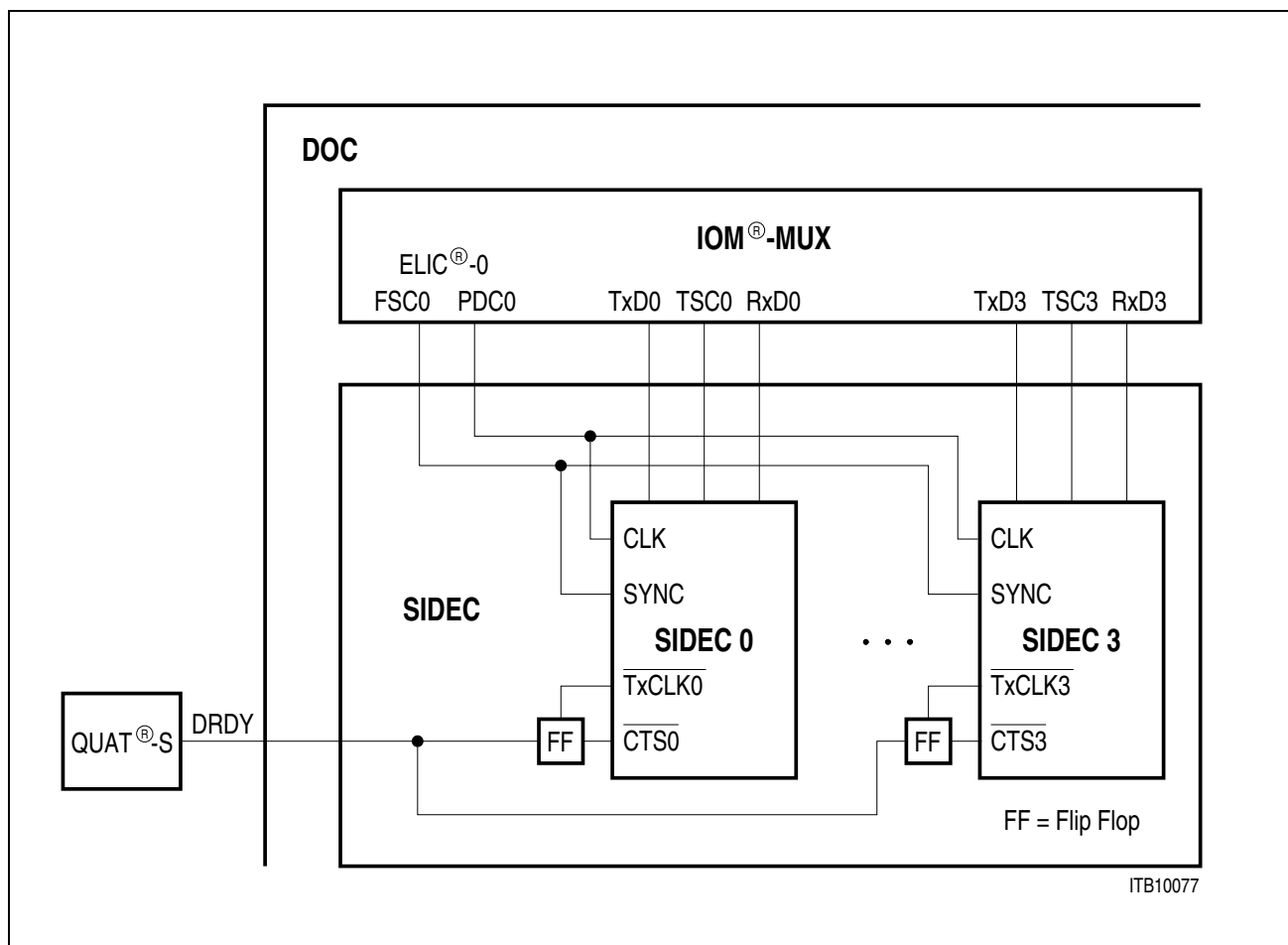
Figure 2-22 SIDEDEC Block Diagram
