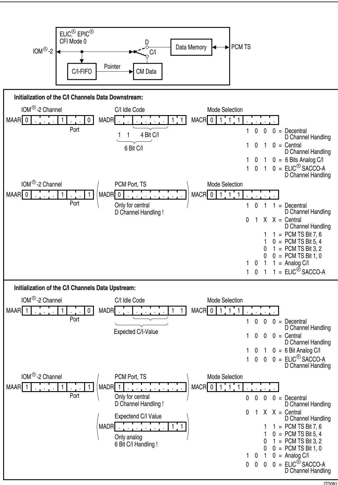
Figure 9-7 Preparing EPIC ® s C/I Channels (working sheet)
