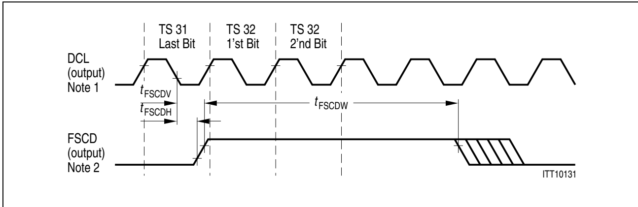
Figure 7-17 FSCD Timing
