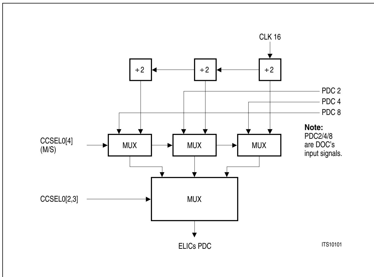
Figure 2-47 PDC Generation
