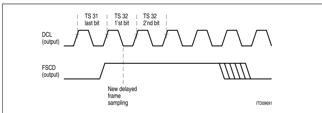
Figure 2-33 FSCD Behavior
