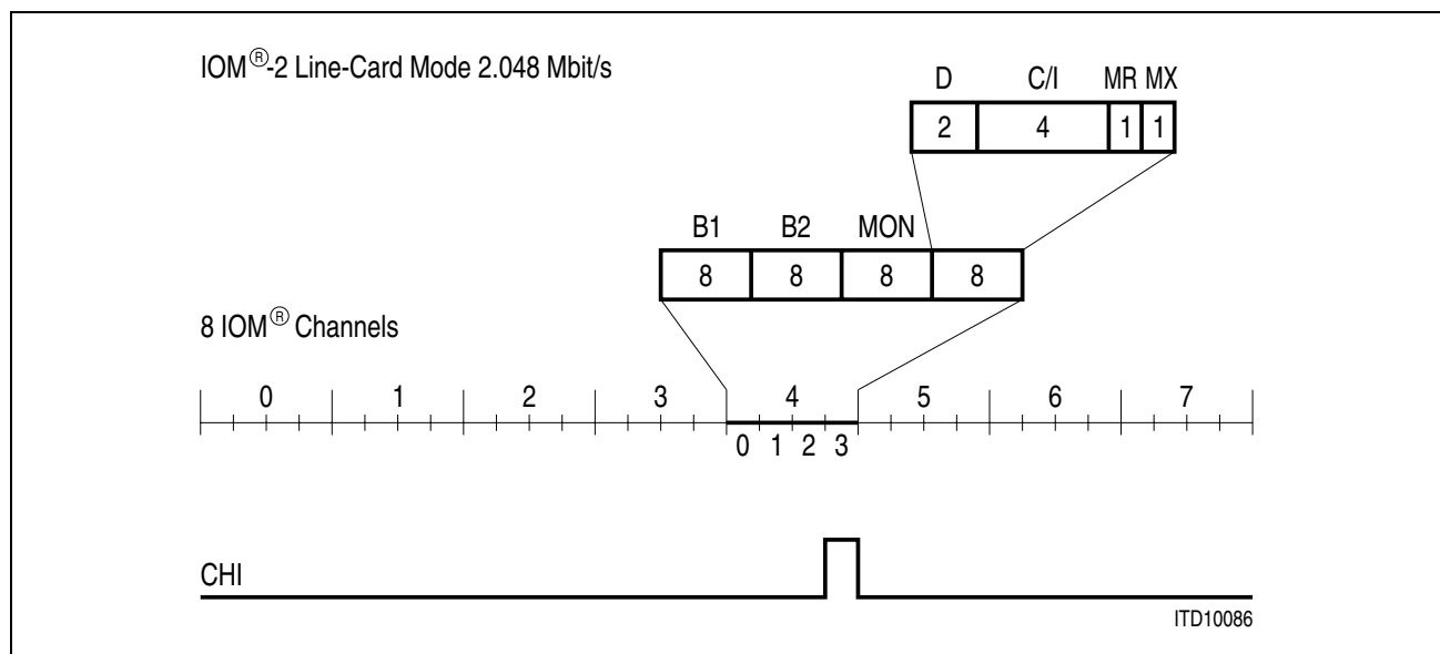
Figure 2-32 CHI Signal
