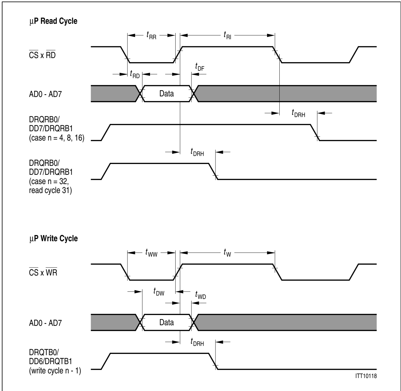
Figure 7-4 Data Timing
