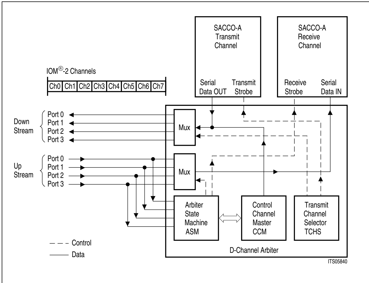
Figure 2-19 D-Channel Arbiter
