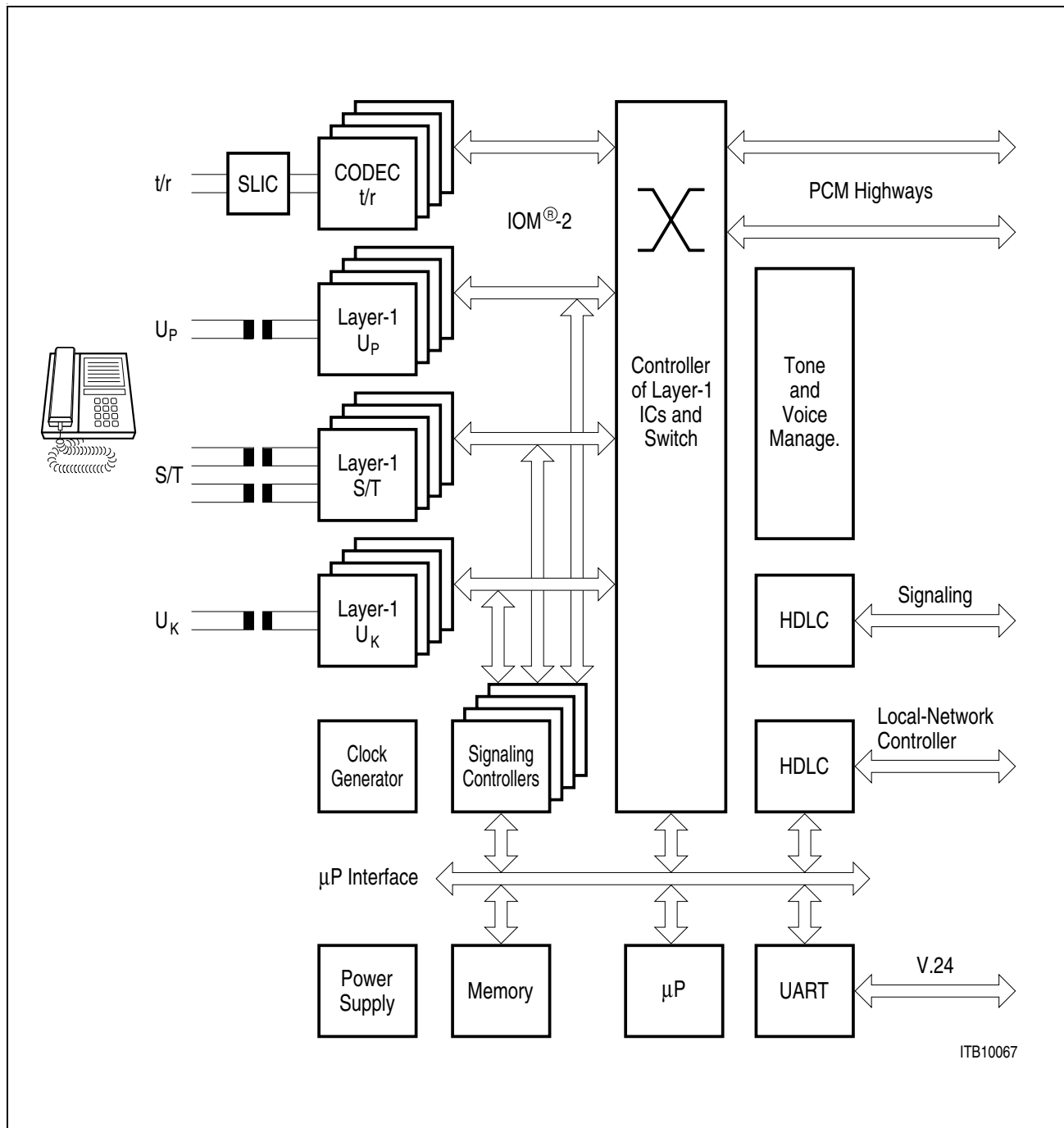
Figure 1-1 Functional Blocks of a PBX
