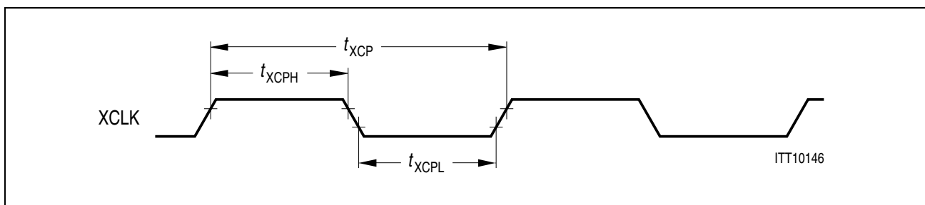
Figure 7-35 XCLK (input) Timing
