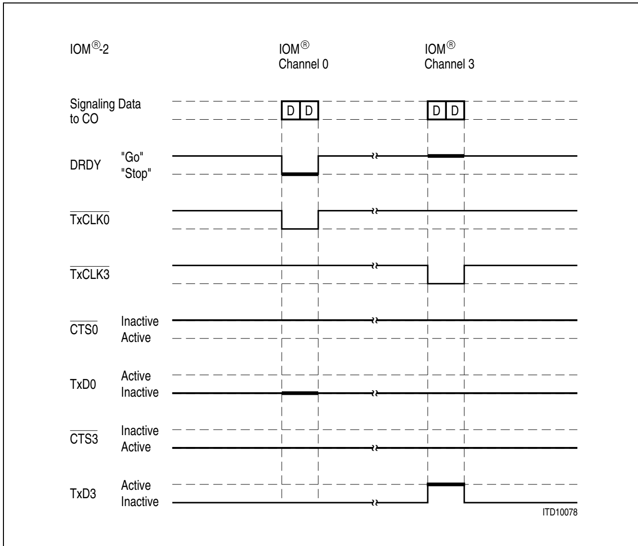
Figure 2-23 SIDECE Signals
