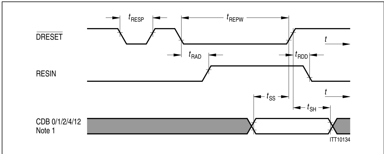
Figure 7-23 DRESET and RESIN timing
