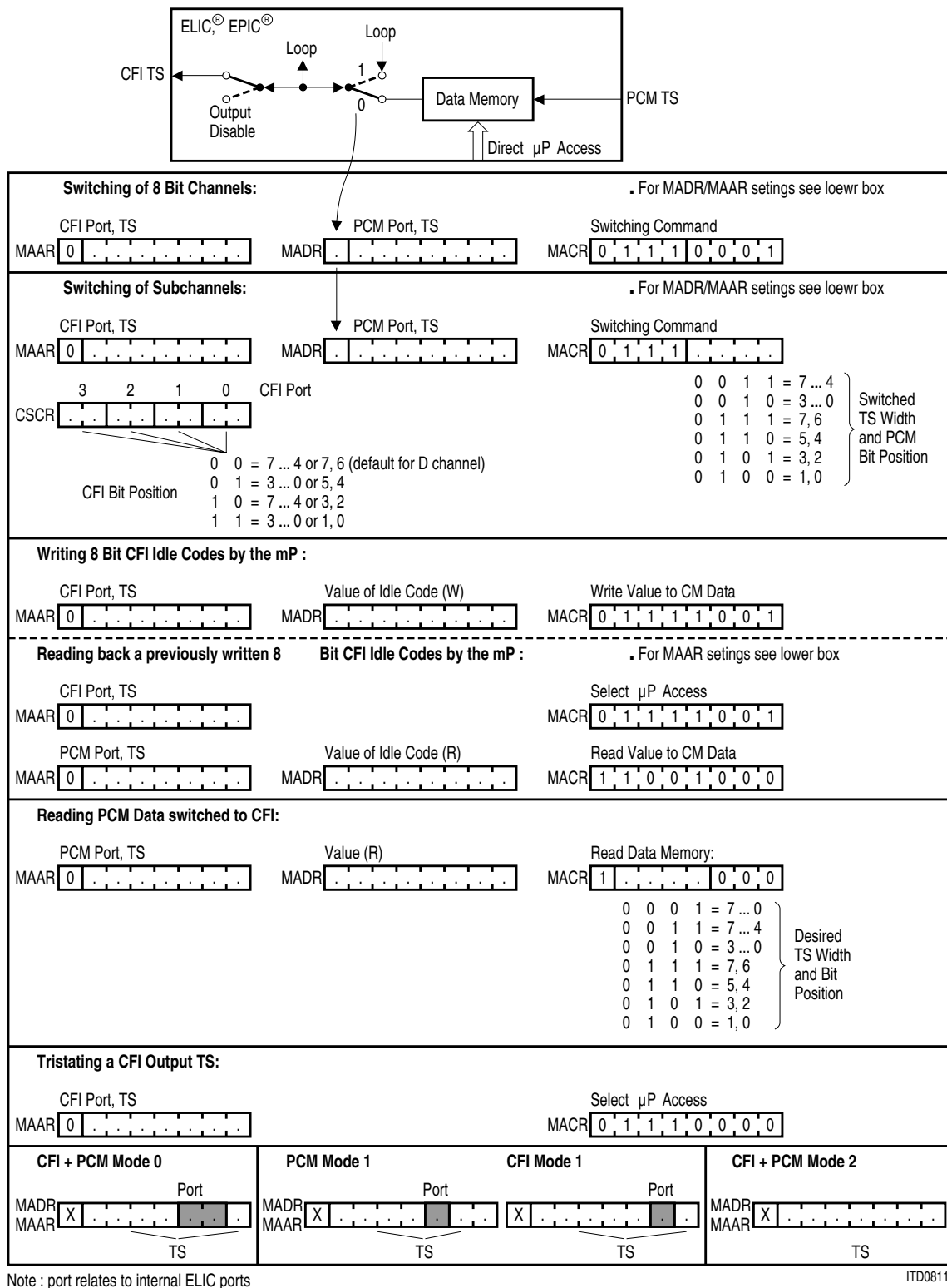
Figure 9-5 Switching of PCM Time-Slots to the CFI Interface (working sheet)
