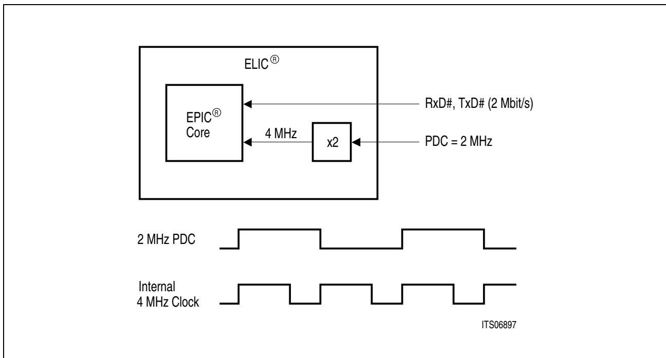
Figure 5-1 Timing Relation Between Internal and External Clock
