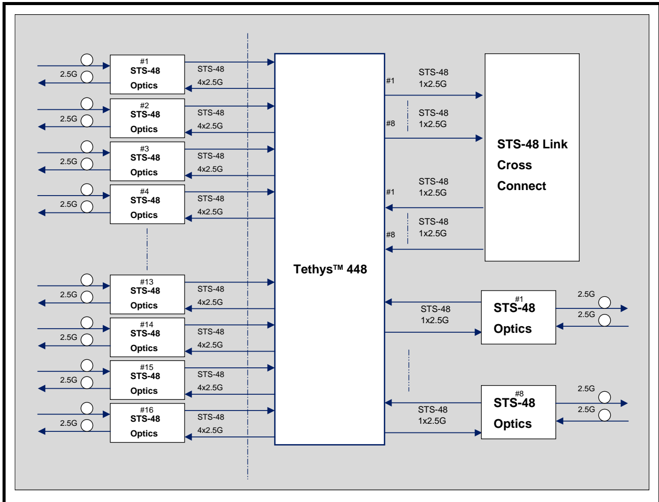
PEB1756E BLOCK DIAGRAM
