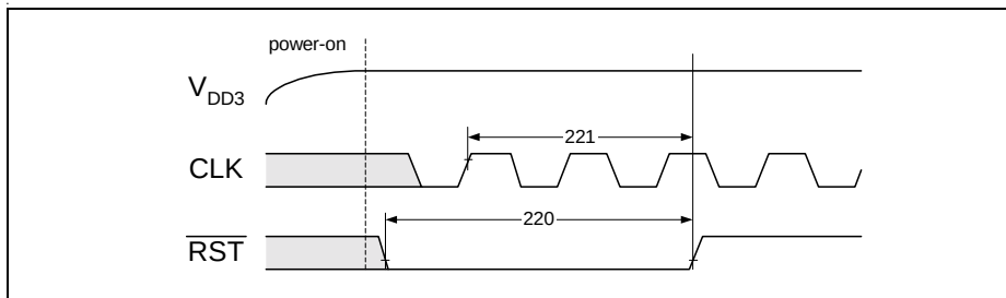
Figure 9-36 Reset Timing
