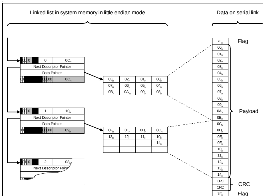
Figure 4-6 Descriptor Structure
