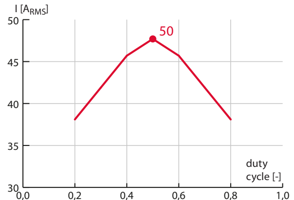
Fig. 4. Current capability as a function of the average duty-cycle
