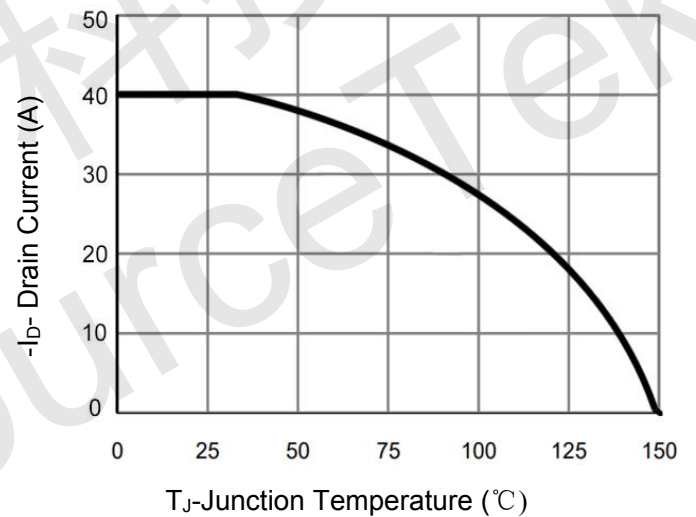
Figure 4 Drain Current
