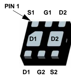
DFN2X2-6L top view
