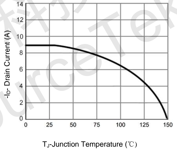
Figure 4 Drain Current
