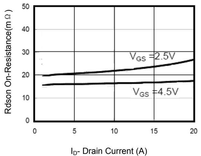
Figure 6 Drain-Source On-Resistance
