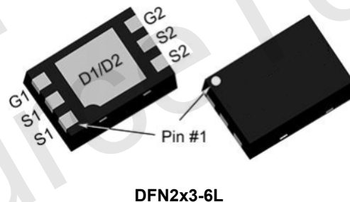
DFN2x3-6L
