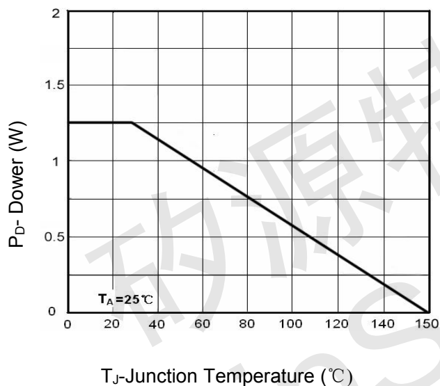
Figure 3 Power Dissipation
