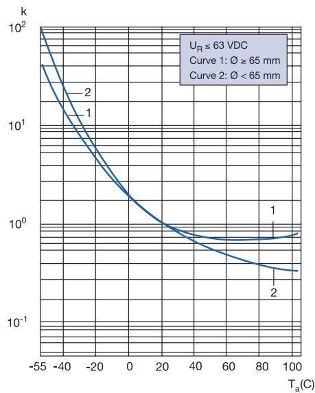
ESR as a function of ambient temperature ( T_a ) at f = 100 kHz. k = R_{ESR}(T_a)/R_{ESR}(20°C)
