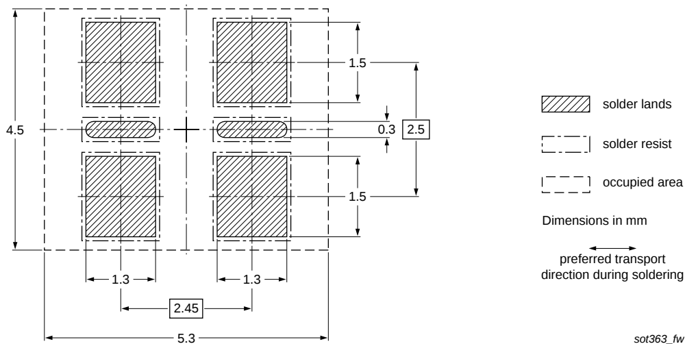
Fig 14. Wave soldering footprint PUMB13 (SOT363)
