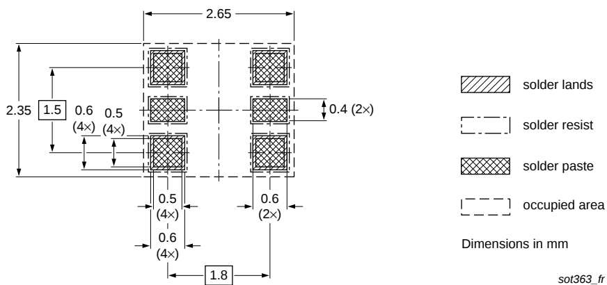
Fig 13. Reflow soldering footprint PUMB13 (SOT363)
