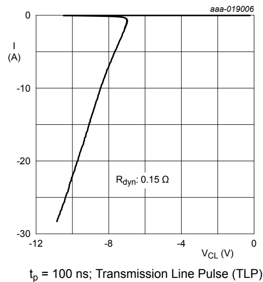
Fig. 6. Dynamic resistance
