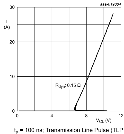
Fig. 5. Dynamic resistance
