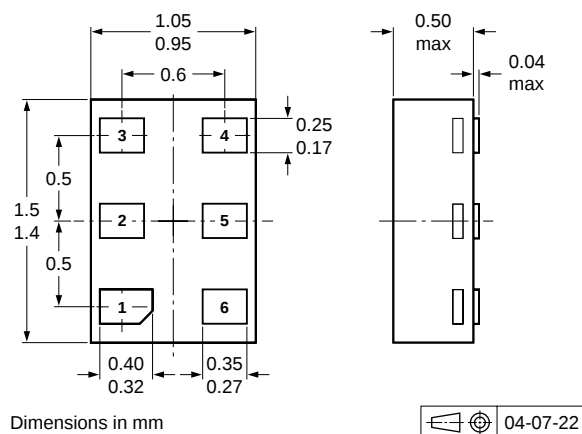
Fig 10. Package outline PESDxV4UF (SOT886)
