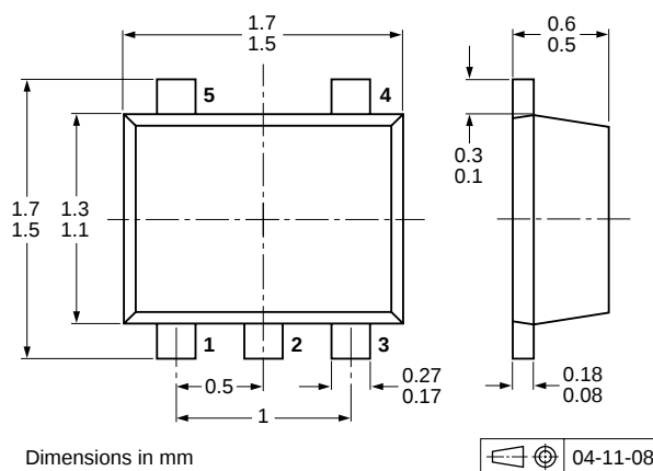
Fig 12. Package outline PESDxV4UW (SOT665)
