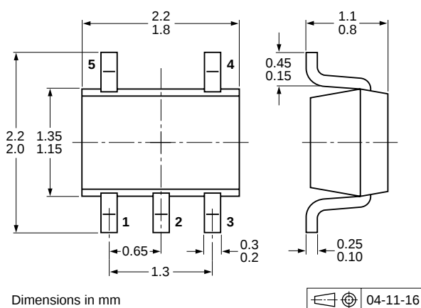
Fig 11. Package outline PESDxV4UG (SOT353)
