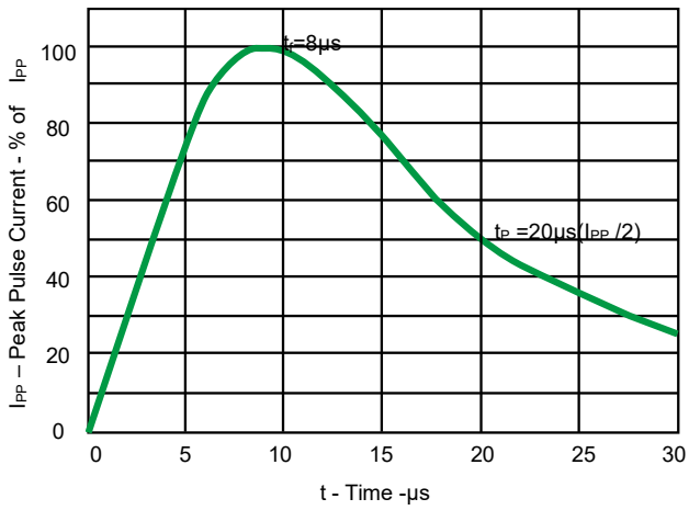
Fig 1. Pulse Waveform
