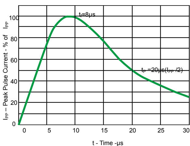
Fig 1.Pulse Waveform
