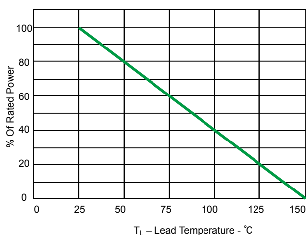
Fig 2.Power Derating Curve
