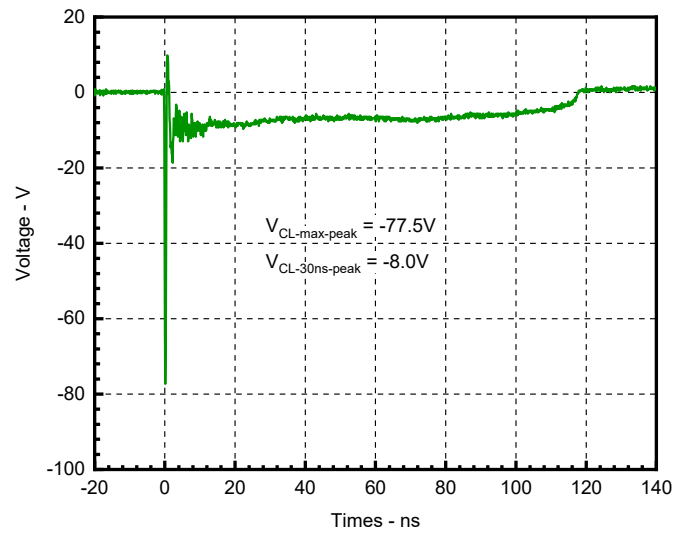
Fig 8. Clamping Voltage at IEC61000-4-2 -8kV Pulse Waveform
