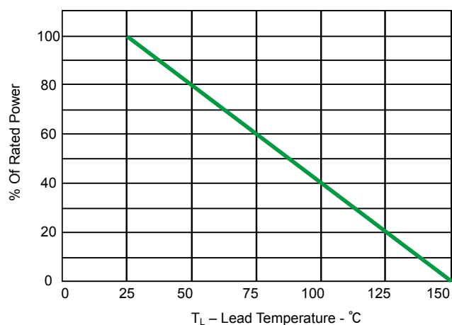
Fig 2.Power derating curve
