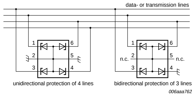
Fig 10. Application diagram
