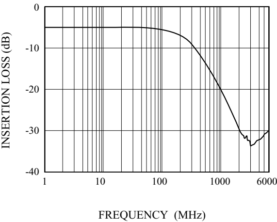
S_{21} - FREQUENCY
