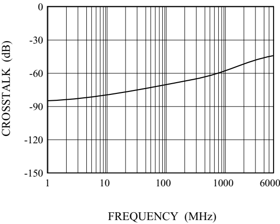
ANALOG CROSSTALK
